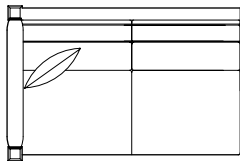
HIGHLANDS LF LOVESEAT 89/91-9800-58-L OUTSIDE W58 D38½ H33½ INSIDE W54 D21 ARM H27½ SEAT H20¼
