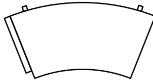
96-9200-L/CI-8200-L High Line Left Arm Facing Section Outside L74 D39½ H33 Inside L57¼ D22¼ Seat H18 Arm H22¼
